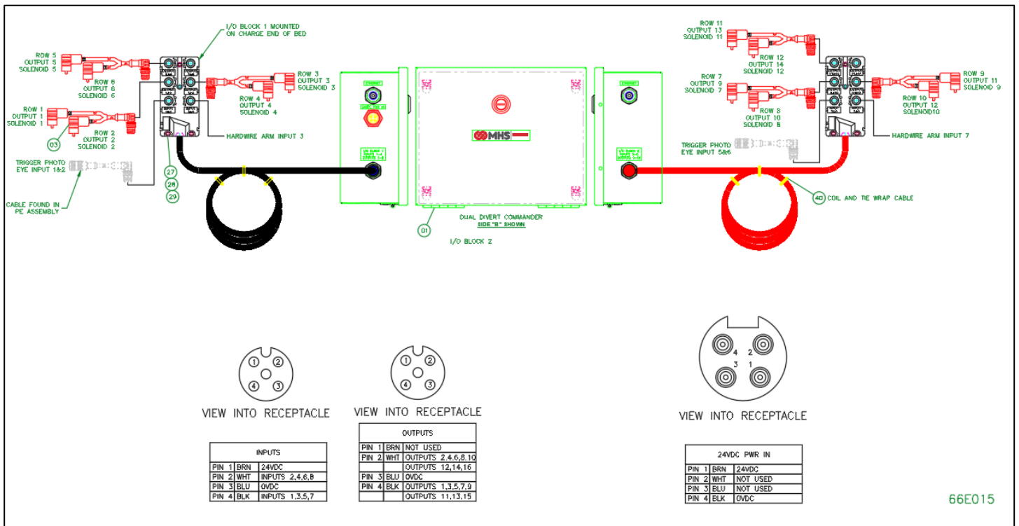
Figure 2: Wave Commander Hardware
